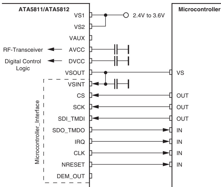
Figure 7-5. 1-Battery Application
